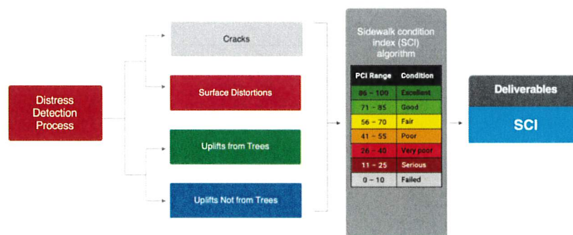
Sidewalk Algorithm
